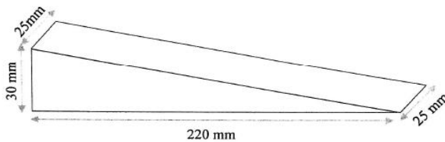
2. PVC WEDGE (220x25x30)
