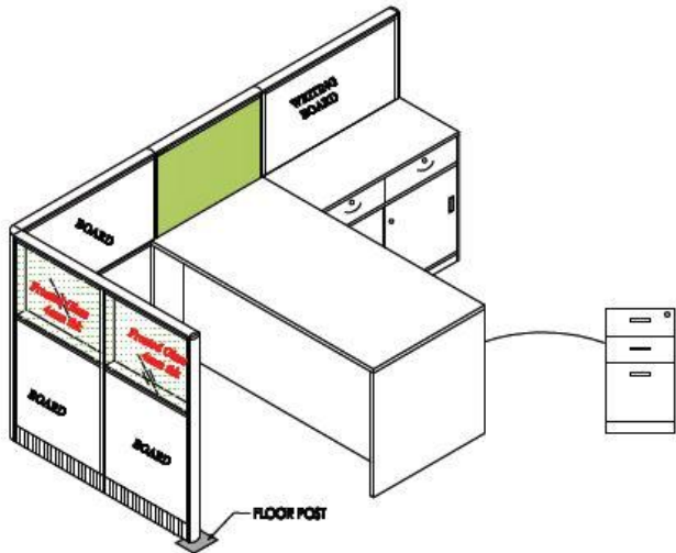
60 MM PRATTION ,TABLE ,FIXED PEDESTAL WITH SIDE UNIT ( AM'S CUBICLE & MANAGER'S CUBICLE )
