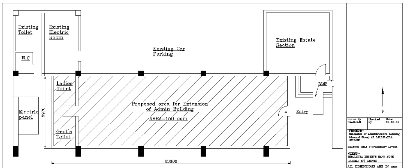
Proposed Area Layout - Plan
