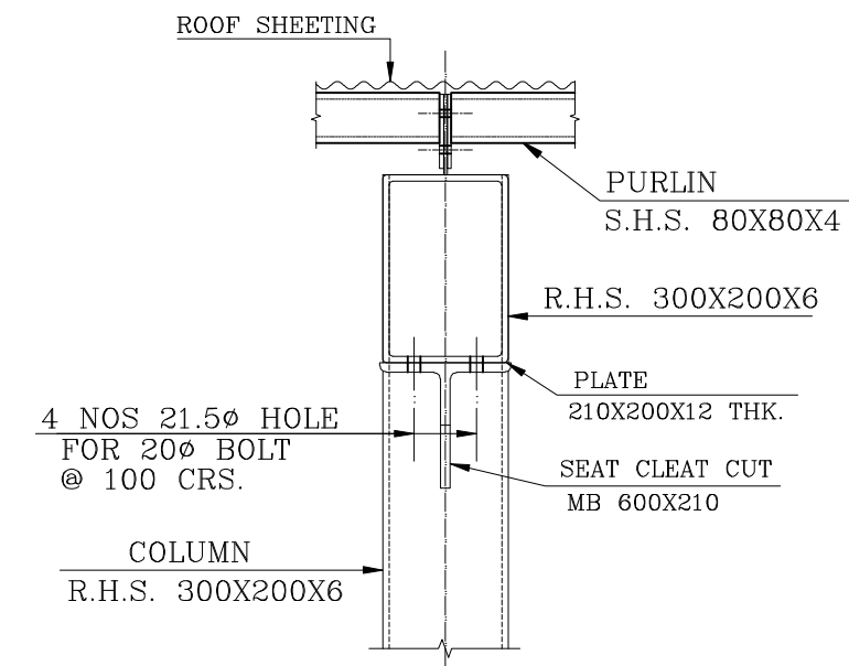
VIEW AT 4-4
