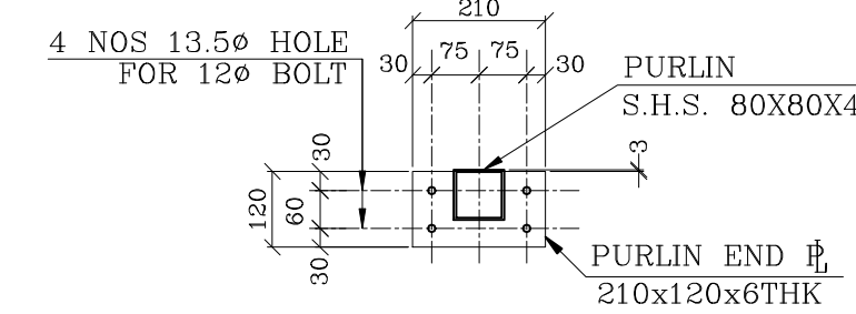
DETAIL OF PURLIN END
