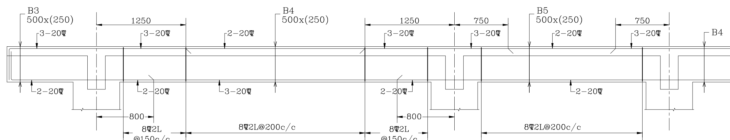
R.C.C DETAILS OF BEAM MKD. B3-B4-B5.
