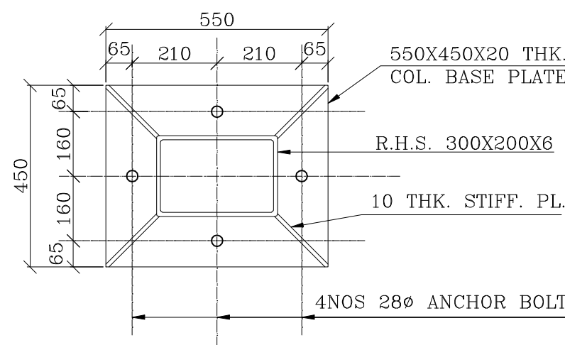
VIEW 3-3 DETAIL OF COLUMN BASE PLATE
