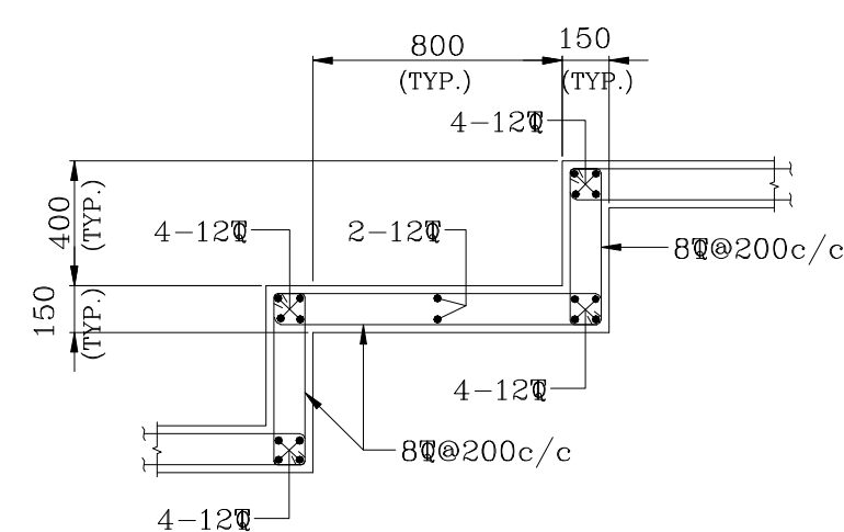
R.C. DETAILS OF GALLERY
