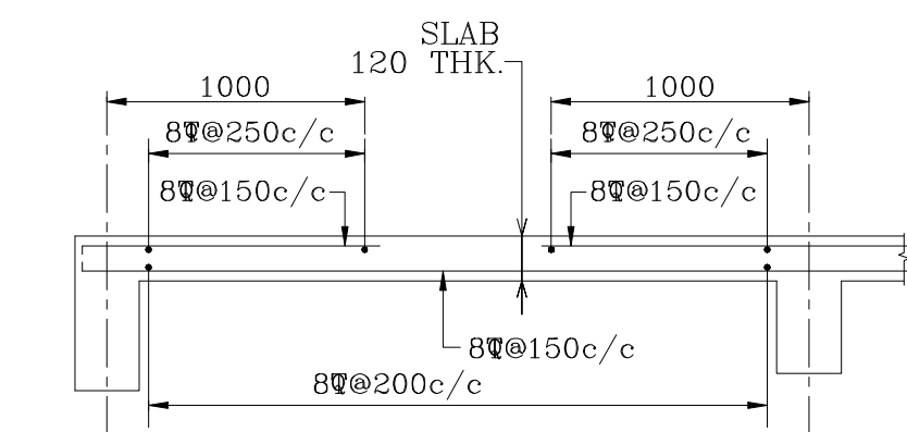
TYPICAL SECTION OF SLAB IN SHORTER SPAN
