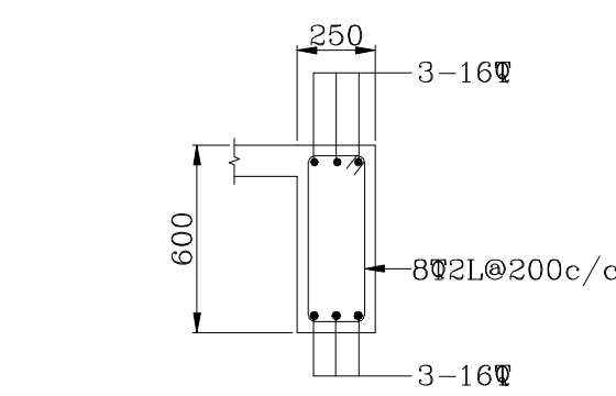
R.C.C DETAILS OF BEAM MKD. B6.
