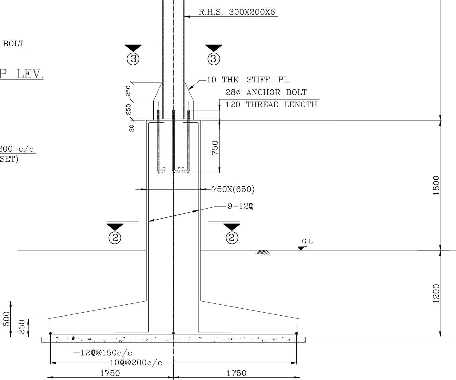
DETAIL OF STEEL COLUMN WITH RAFTER AND FOUNDATION
