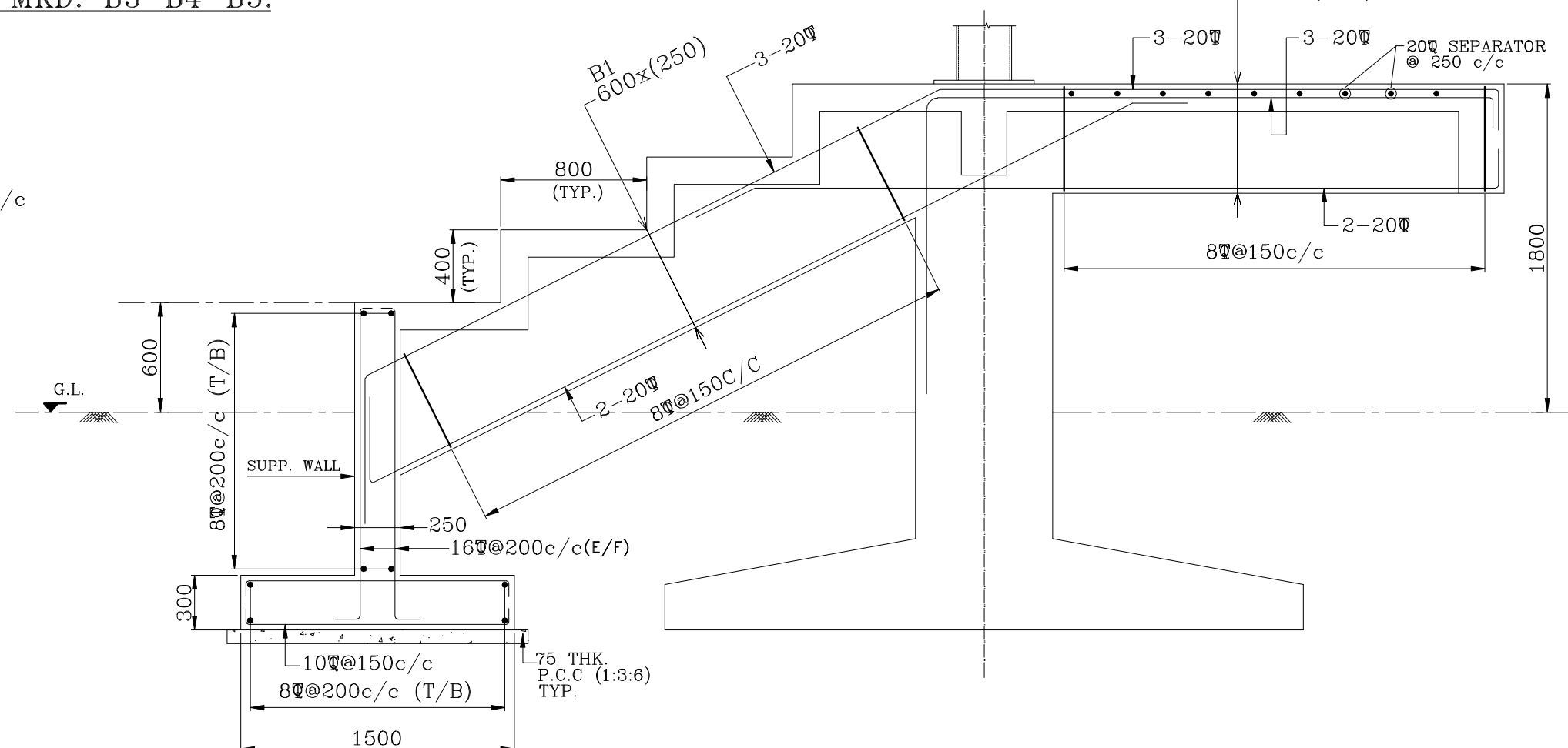
R.C.C DETAILS OF BEAM MKD. B1-B2.
