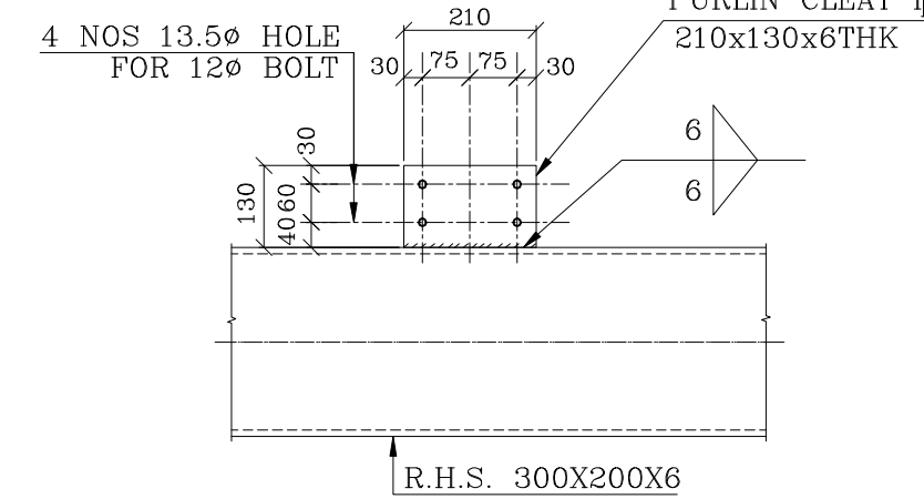
DETAIL OF PURLIN CLEAT
