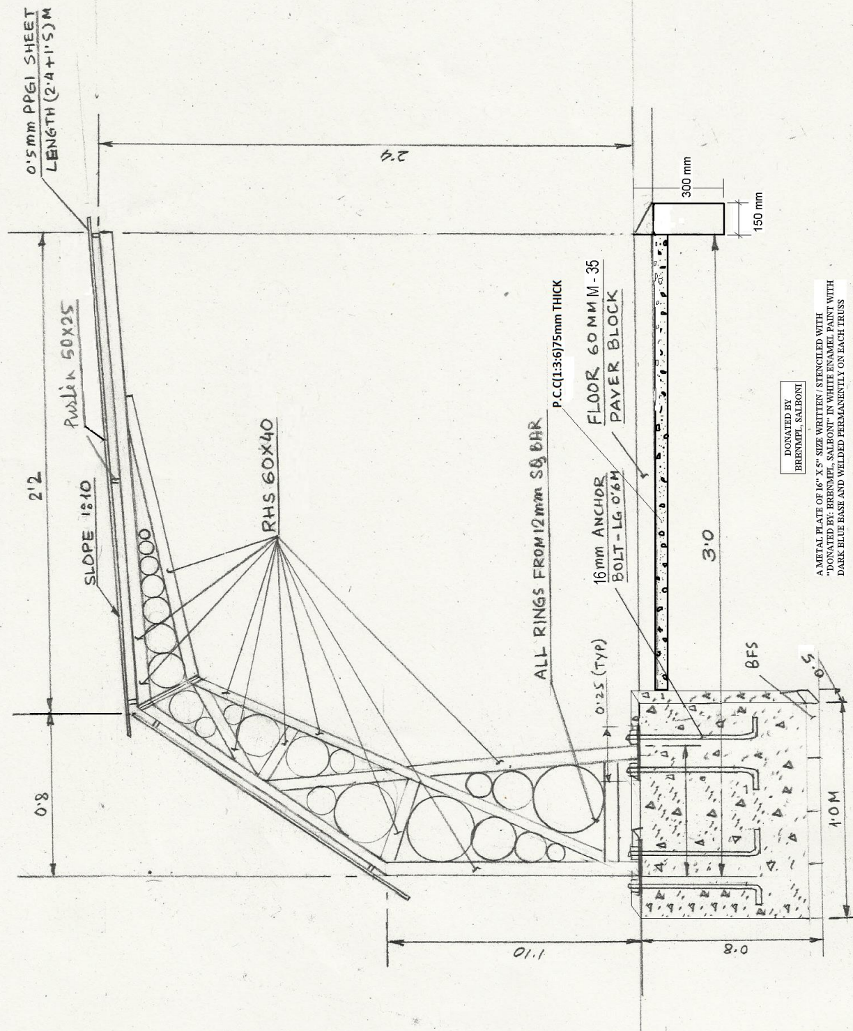
STRUCTURAL DRAWING OF BI-CYCLE SHED
