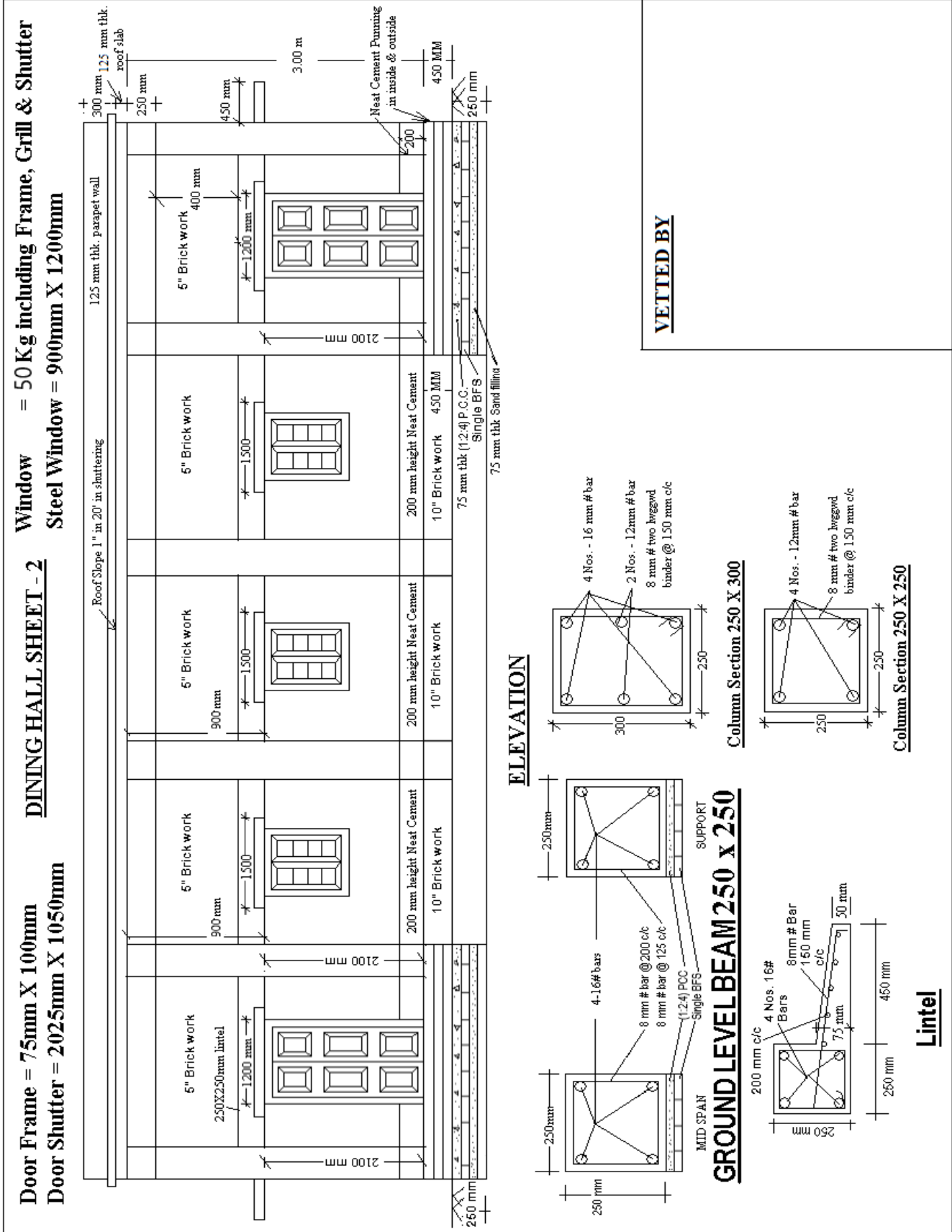
Drawing- 2/2
