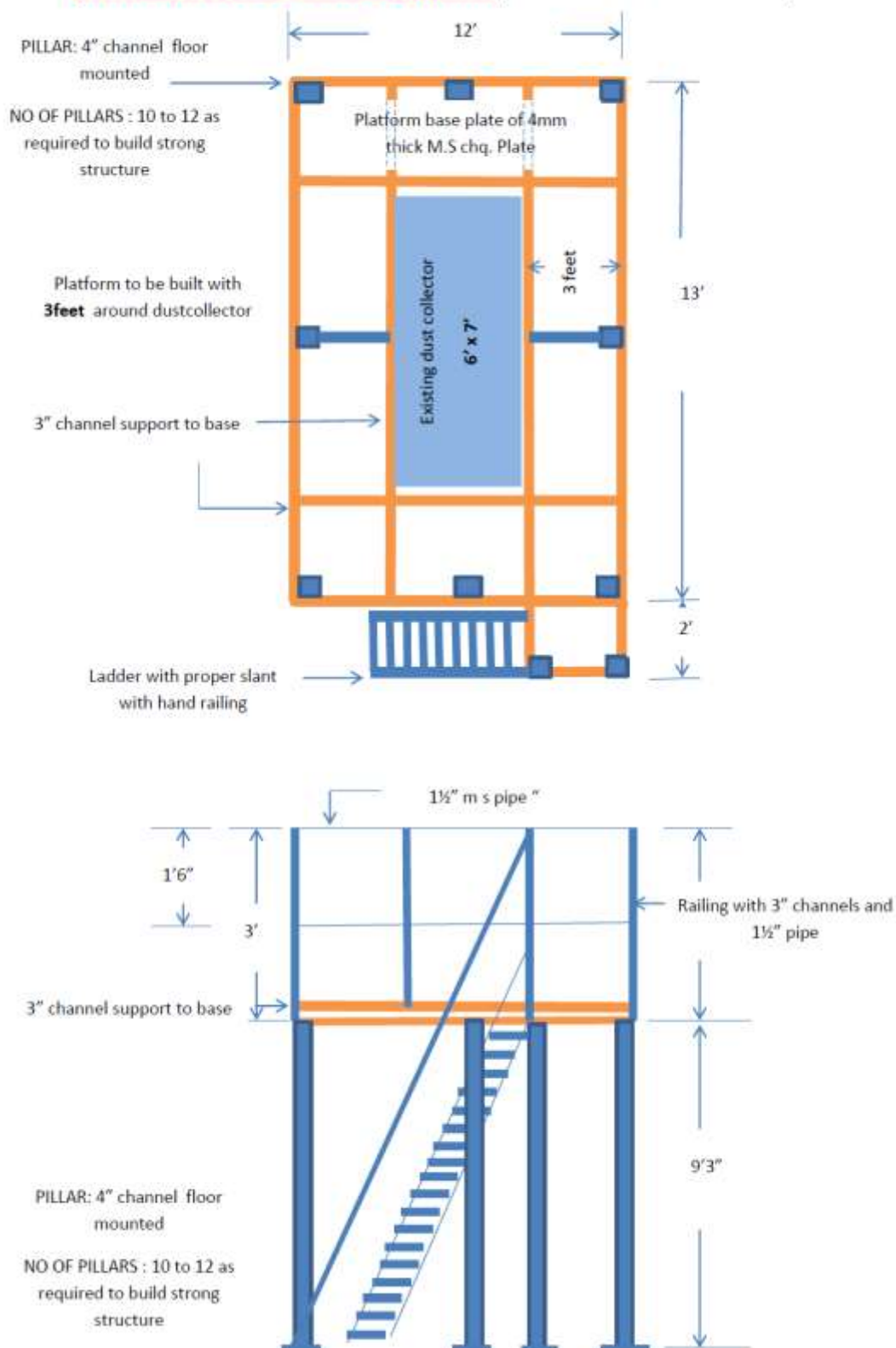
SKETCH FOR DUST COLLECTOR PLATFORM (NOT TO SCALE - Dimensions are in inches)
