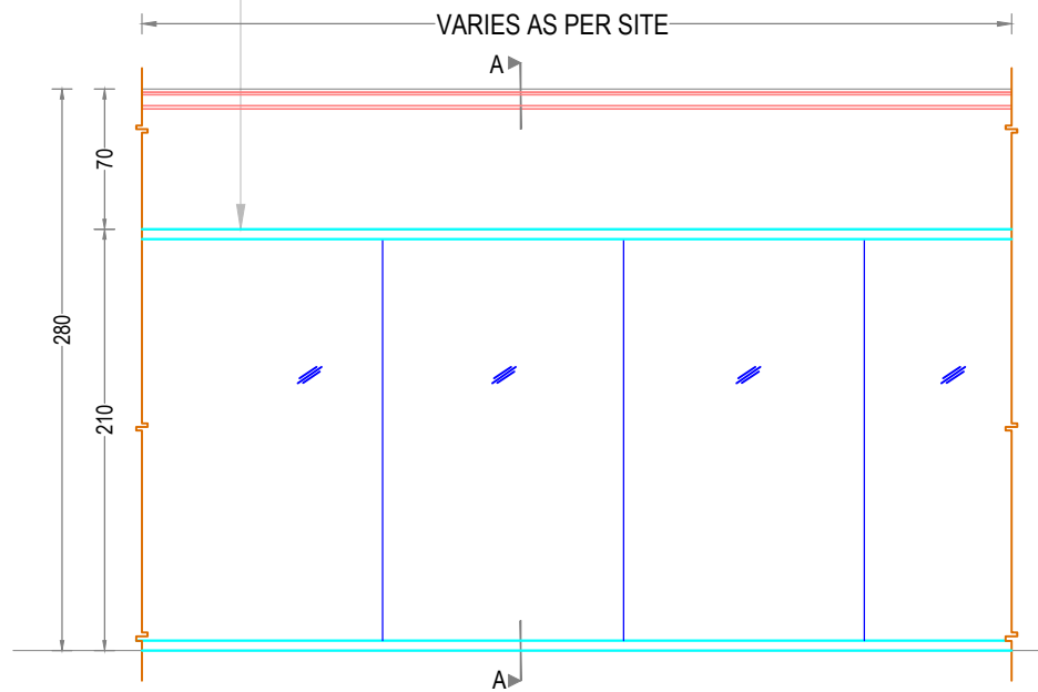
FULL HEIGHT GLAZED PARTITION
