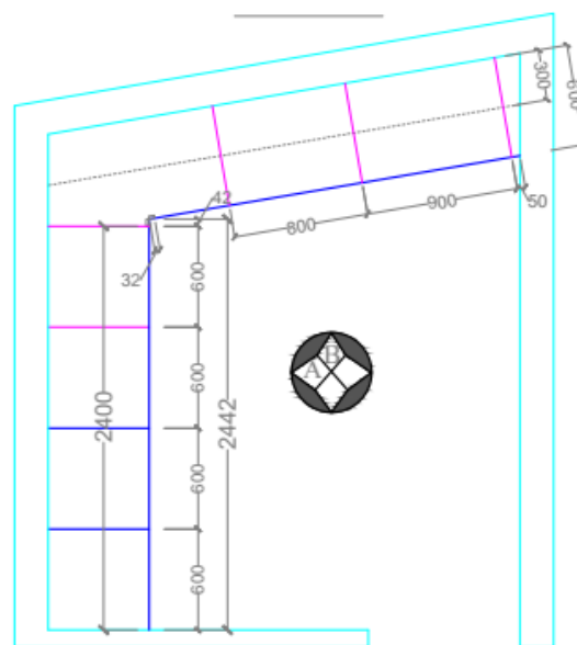
PANTRY LAYOUT
