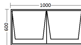
W8a - 4 Nos 2 Panel Top Hung
