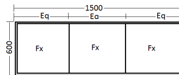
W6 - 4 Nos 3 Panel Fixed Window
