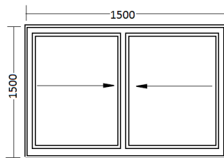
W5 - 10Nos 3 Track 2 Panel Sliding Window With Mesh
