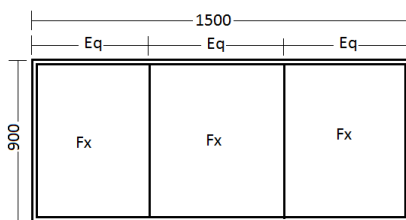
W7 - 9 Nos 3 Panel Fixed Window
