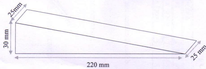
2. PVC WEDGE (220x25x30)
