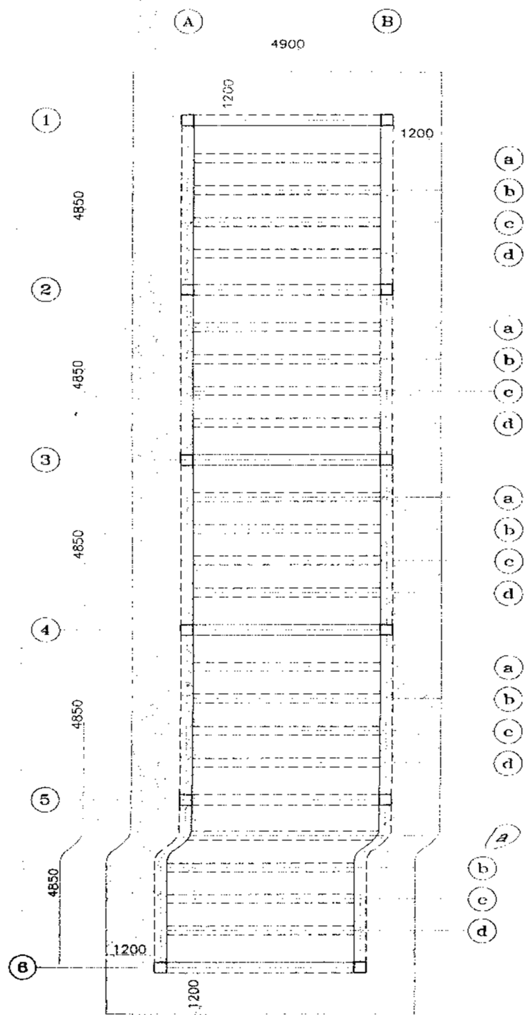
LAYOUT OF COLUMN & BEAM
