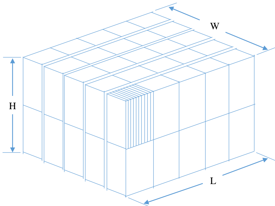
Arrangement of 5 Mini-packs inside Box
