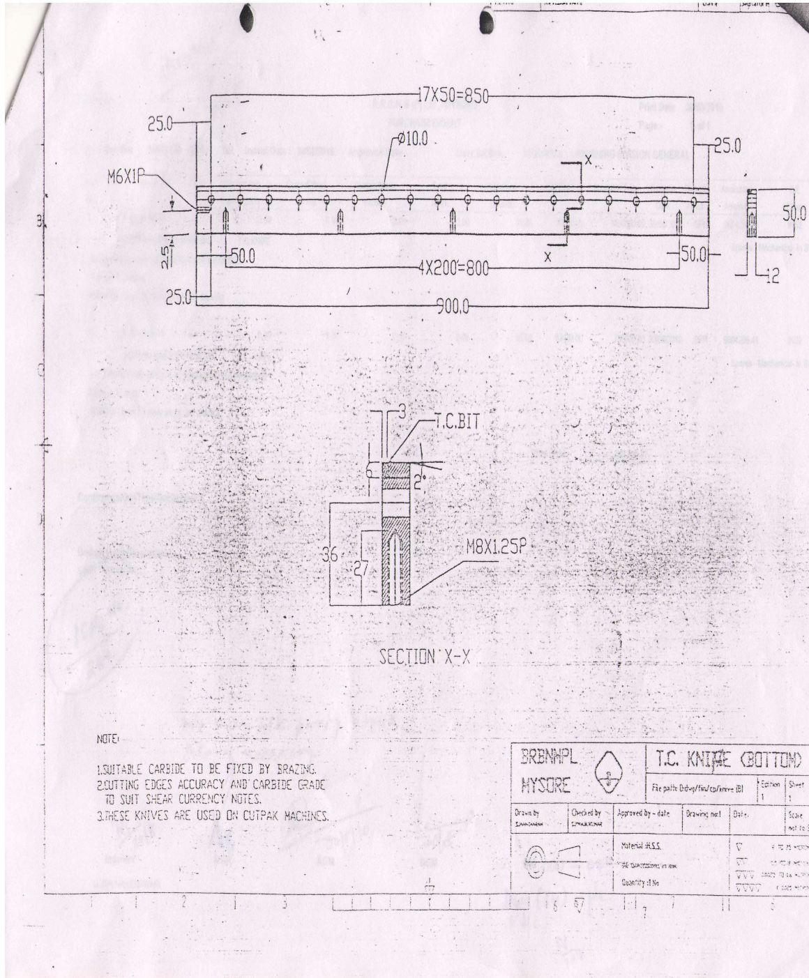
Drawing of Bottom Knife (Tungsten Carbide Knife) for Cutpak machines Size: 900mm x 50mm x 12 mm
