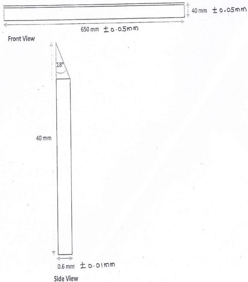
Schematic Drawing of Scraper Knife 40/0.6 X 650
