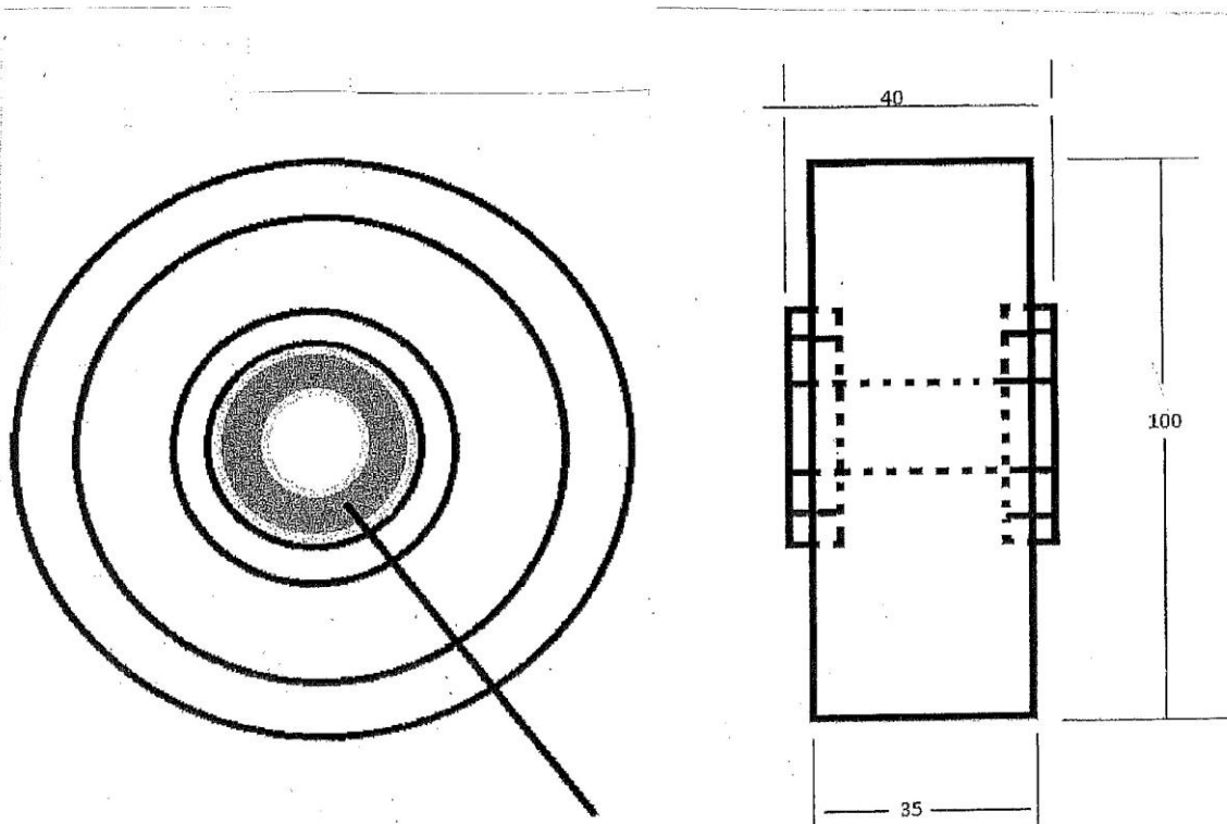
Bearing No.6201 R S
