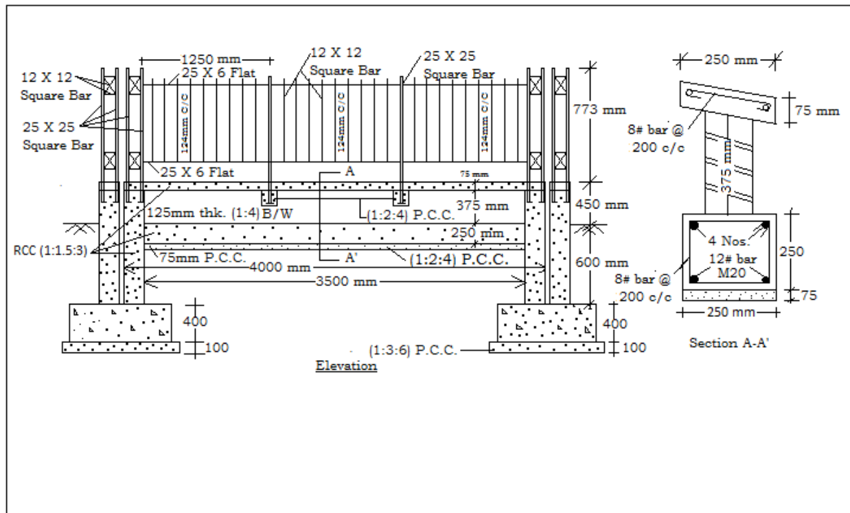
II-2: Elevation showing Grill details
