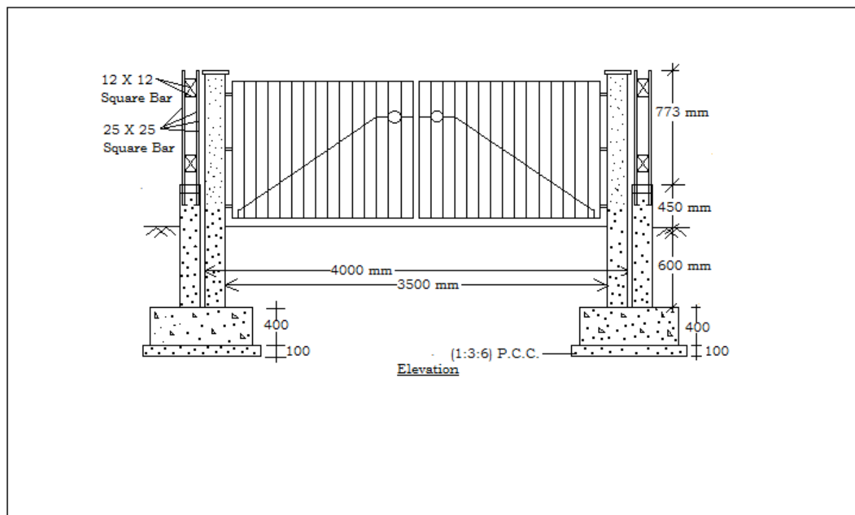
II-3: Elevation showing Gate Details
