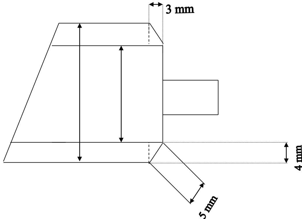
(Diagram for chamfer to be given for Rollers)
