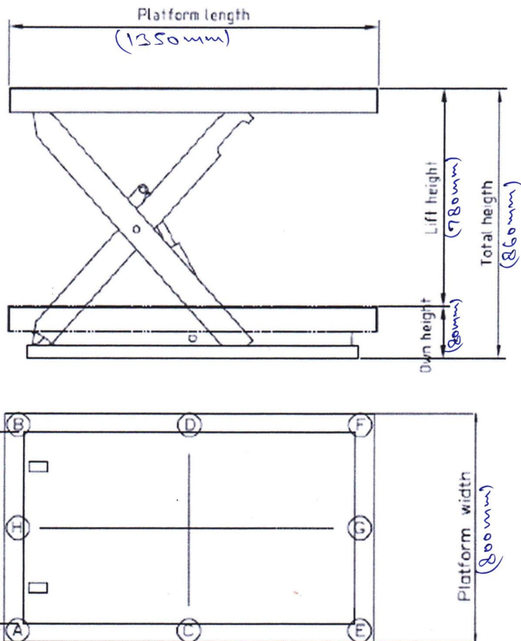
Diagram for Scissor Lift Table:
